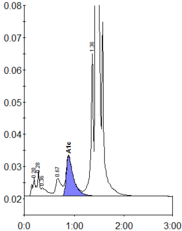
Peak table - ID: 10453972
